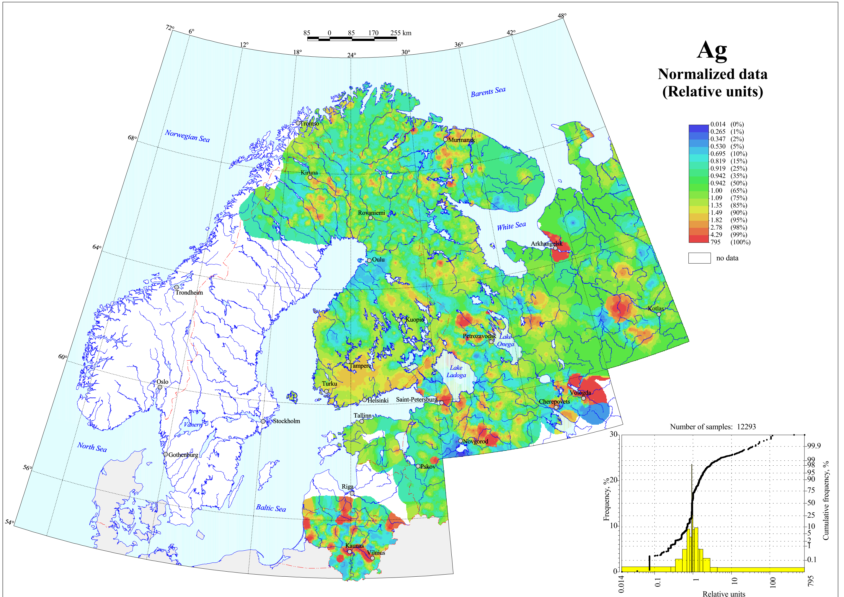
Silver in Stream Sediment
